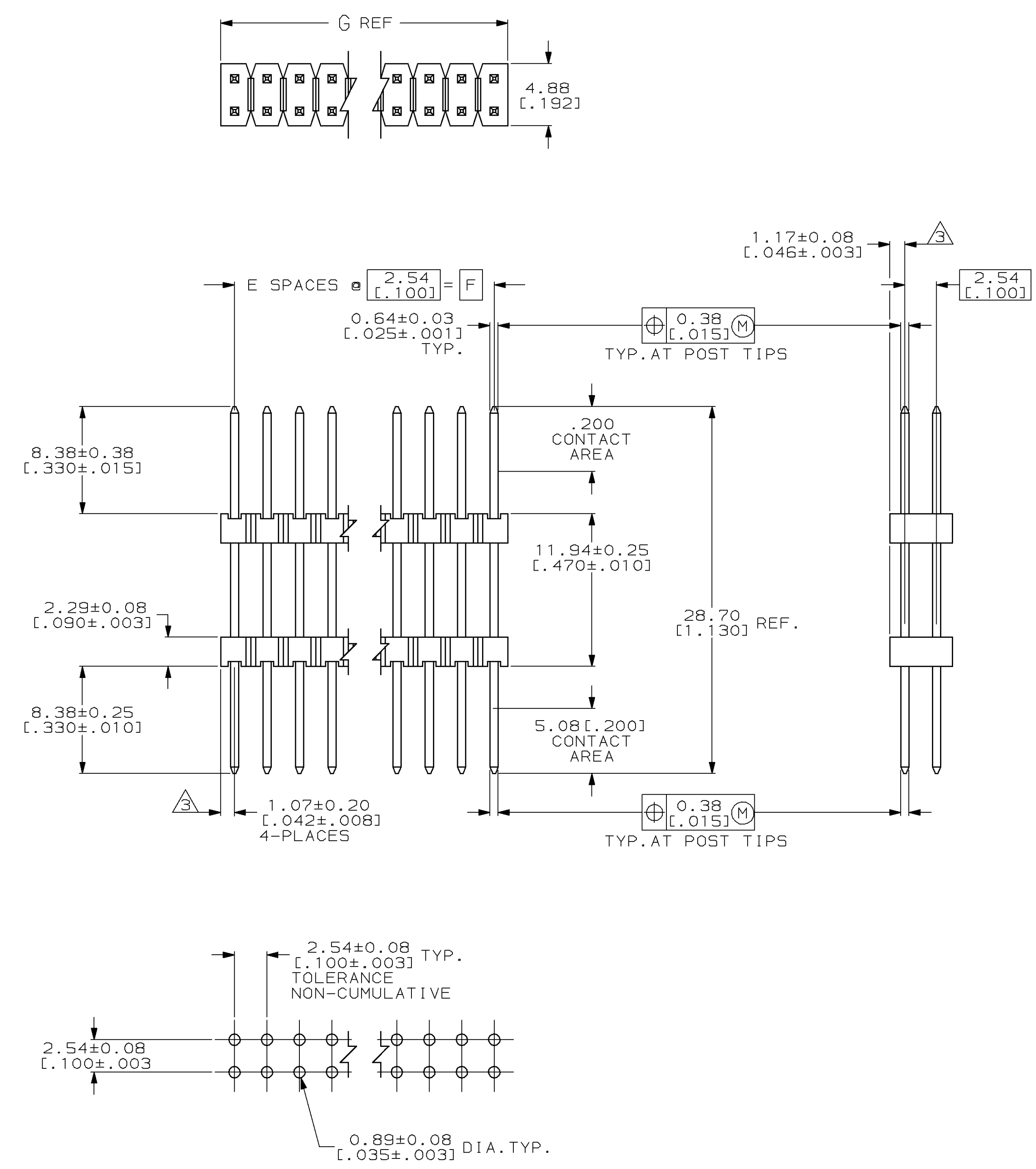
RECOMMENDED HOLE LAYOUT
